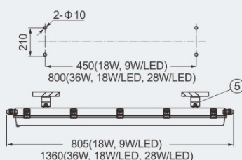
X: ceiling type
