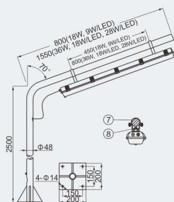
Suitable for ground pole type
