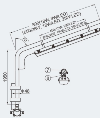
Suitable for fence pole type
