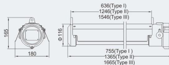
BAY51-D-□□x□□ With external reflector
