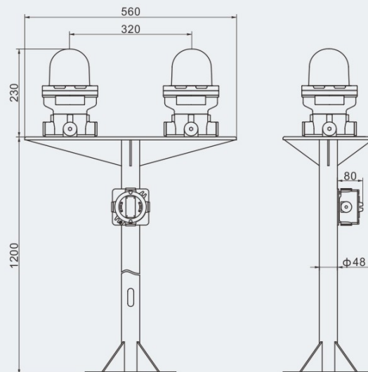
Drawings of main (spare) caution spotlight fittings
